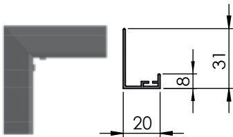
M - Medium Border with 20 mm
