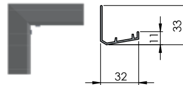
A - Angled Border with 32 mm
