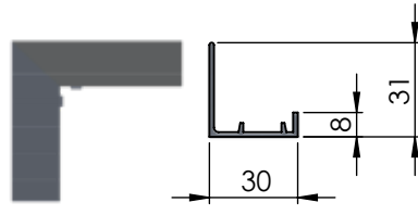
L - Large Border with 30 mm
